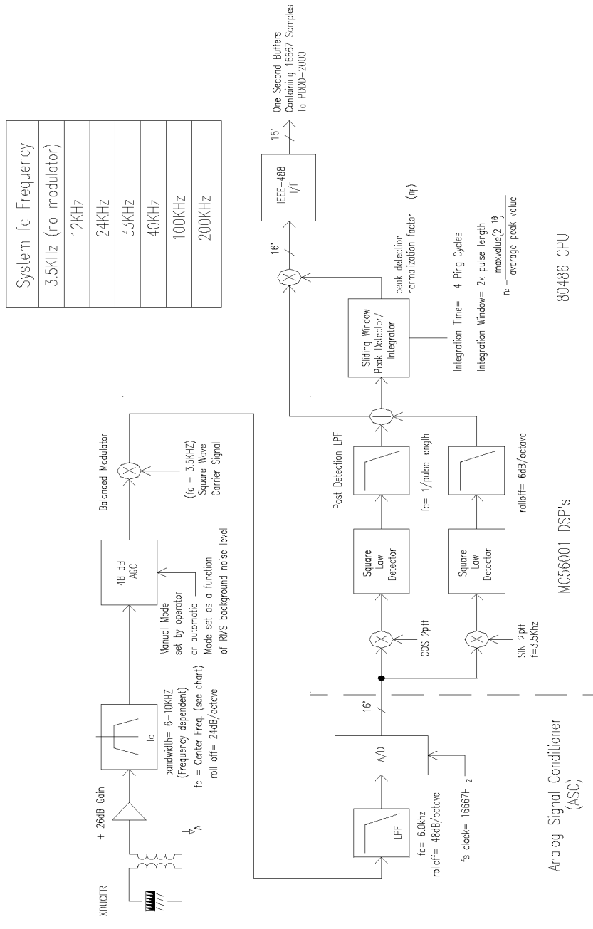
Figure 6-1 12kHz CW DETECTION PROCESSING
